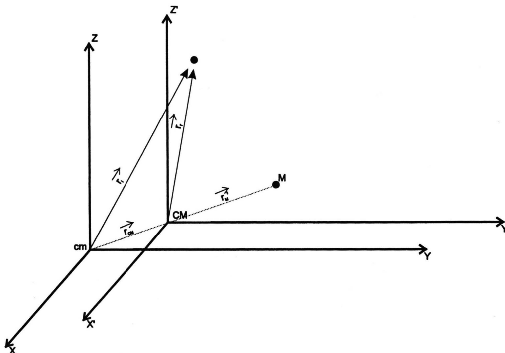
Fig. 1. Principal axis system ( x, y, z ; cm) of the asymmetric top base molecule and an axis system ( x', y', z' ; CM) originating in the center of mass (CM) of the complex. The axes x and x' , y and y' , z and z' are parallel. \mathbf{r}_M = \mathbf{r}_{CM} + \mathbf{r}'_M is colinear with \mathbf{r}_{CM} and \mathbf{r}'_M .
